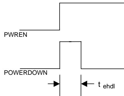
Figure 7-9. Power Enable to Power Down
