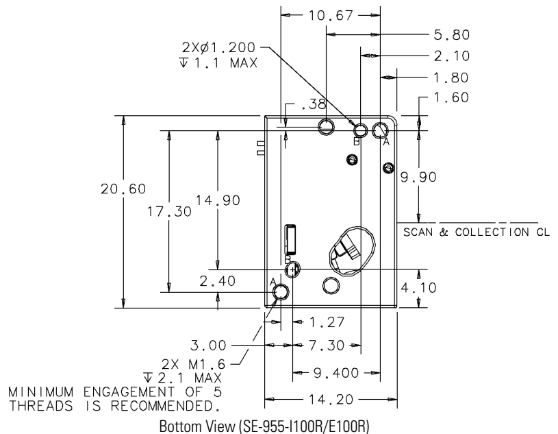
Figure 2-1. SE-955 Mounting Diagram
