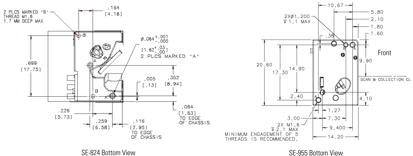
Figure 3-1. SE-824 vs. SE-955 Mounting Diagram
